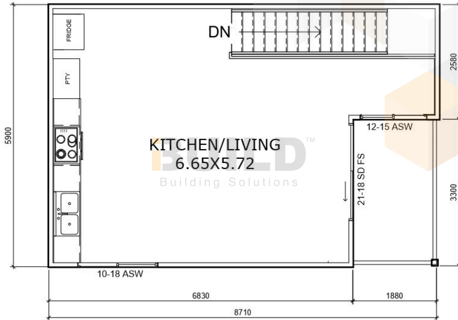
FIRST FLOORPLAN
